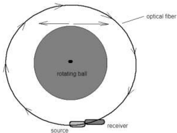
Figure 3: Doppler effect and rotating dark energy
